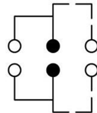
SCHEMATIC (NON-SHORTING)
